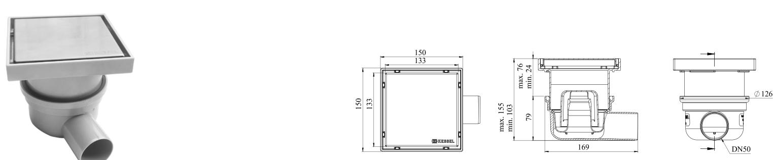
375020016 Point Drain with Tileable Cover
