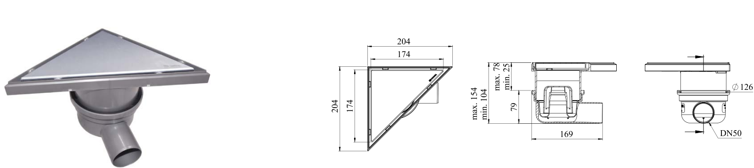
375020017 Corner Shower Drain
