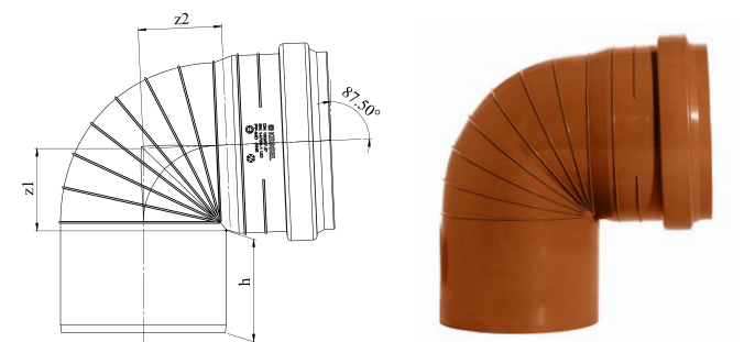
Bend 87.5°
