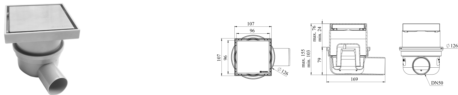
375020015 Point Drain with Tileable Cover
