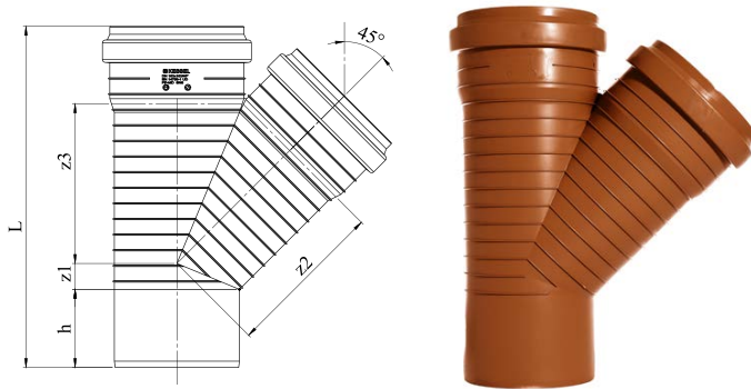
Branch 45°
