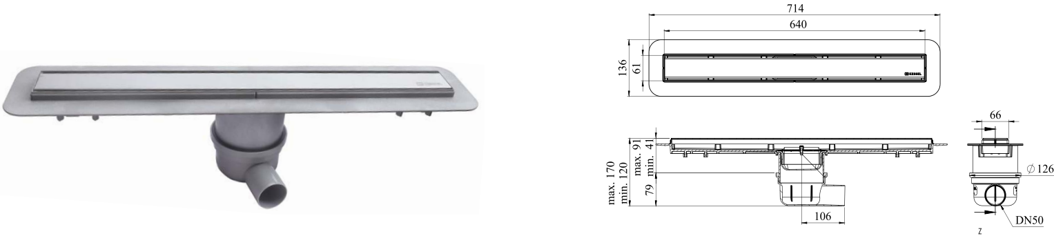
375020012 Shower Channel 650 mm
