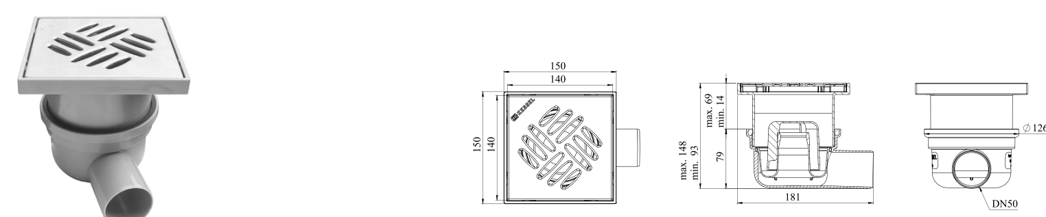
375020014 Point Drain with Open Cover
