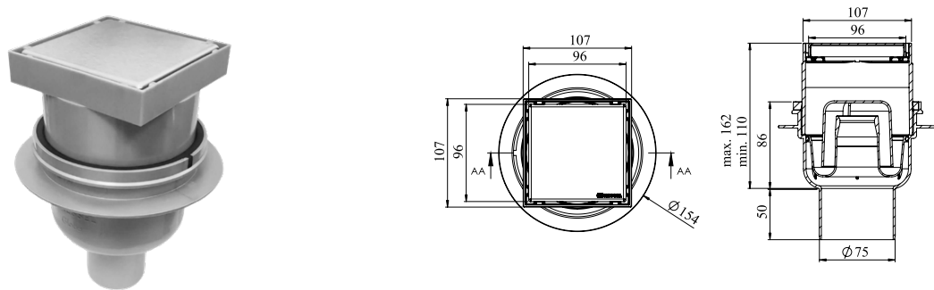
375020036 Point Drain with vertical outlet
