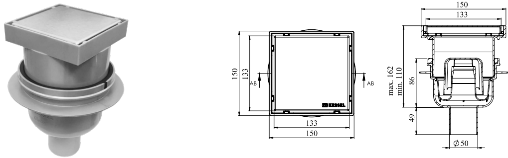
375020035 Point Drain with vertical outlet
