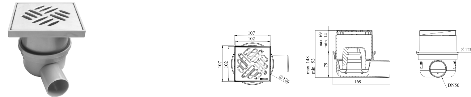
375020013 Point Drain with Open Cover
