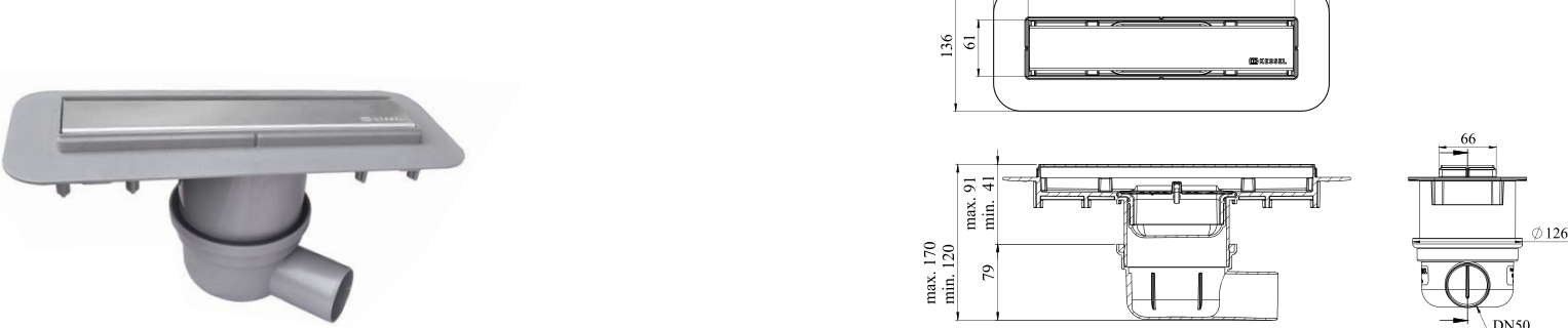
375020011 Shower Channel 300 mm
