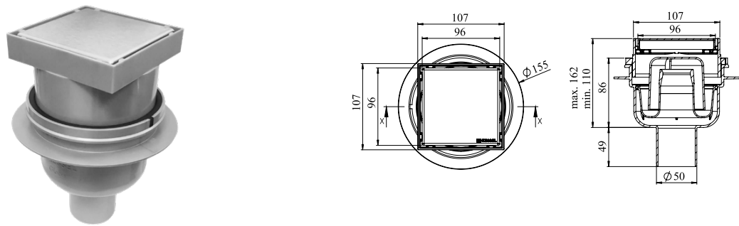
375020037 Point Drain with vertical outlet
