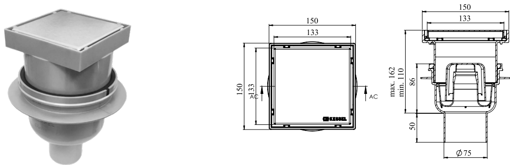
375020034 Point Drain with vertical outlet
