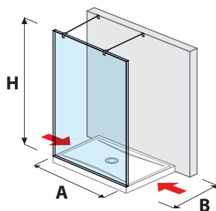
glass wall PURE fixed 120, 130, 140 cm
