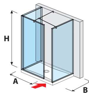
glass wall/walk in PURE for shower trays 80 × 80 cm | 80 × 90 cm
