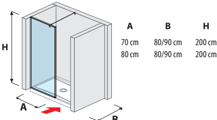
glass wall side-mounted 70, 80 cm
