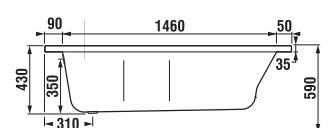
bathtub for installation with panel
