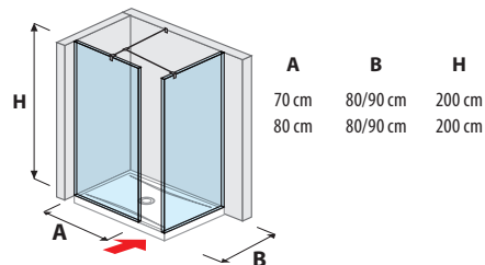
wall/walk in corner version for a shower trays 70, 80 x 80 cm and 70, 80 x 90 cm
