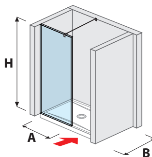
glass wall PURE side-mounted 70, 80 cm
