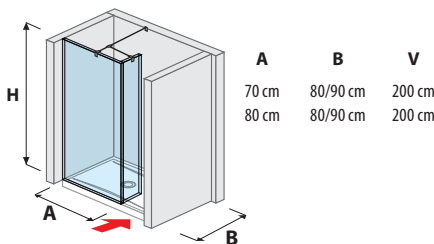
glass wall incl. short glass 70, 80 cm
