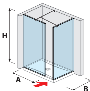
glass wall/walk in PURE corner version for shower trays 70, 80 × 80 cm | 70, 80 × 90 cm
