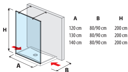
glass wall fixed 120, 130, 140 cm
