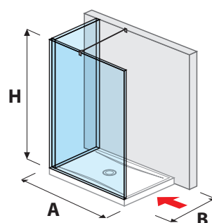
glass wall PURE „L“ 120 × 80 cm | 120, 140 × 90 cm
