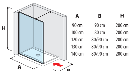
glass wall side-mounted 90, 100, 120, 130, 140 cm
