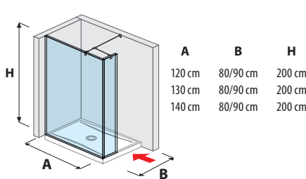
glass wall incl. short glass 120, 130, 140 cm
