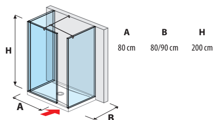
glass wall/walk in for a shower trays 80 x 80 cm and 80 x 90 cm
