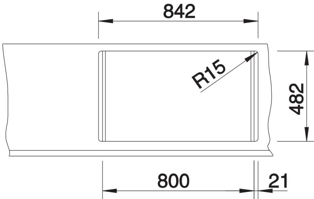
Cut-out
